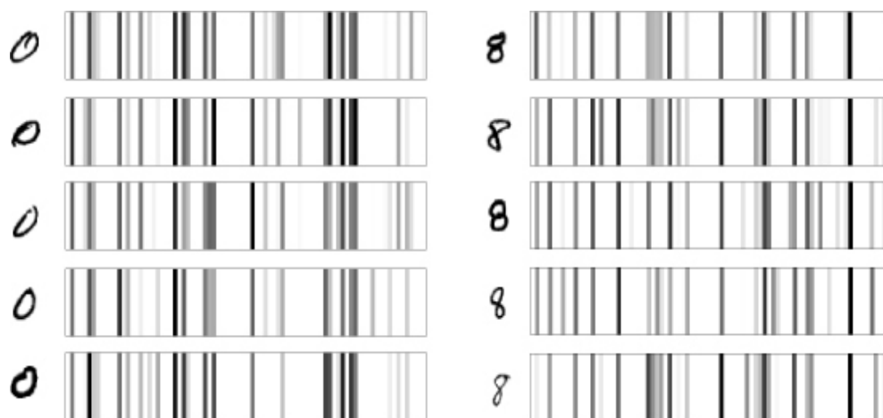
Figure 5-7: Dense layer output for sample inputs
