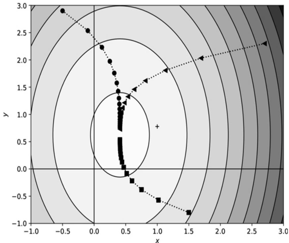
Figure 4-5: Gradient descent in two dimensions
