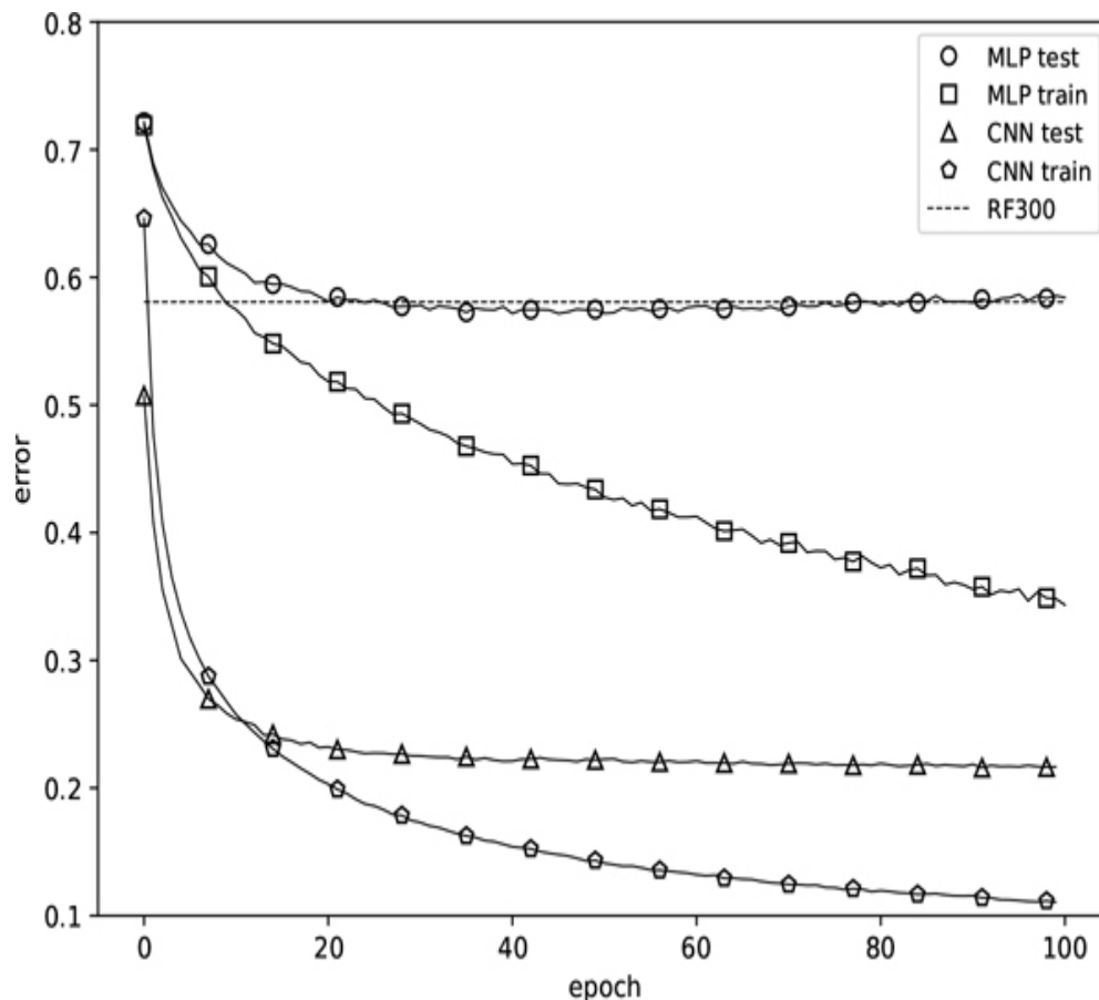
Figure 5-9: CIFAR-10 results for a CNN, MLP, and random forest
