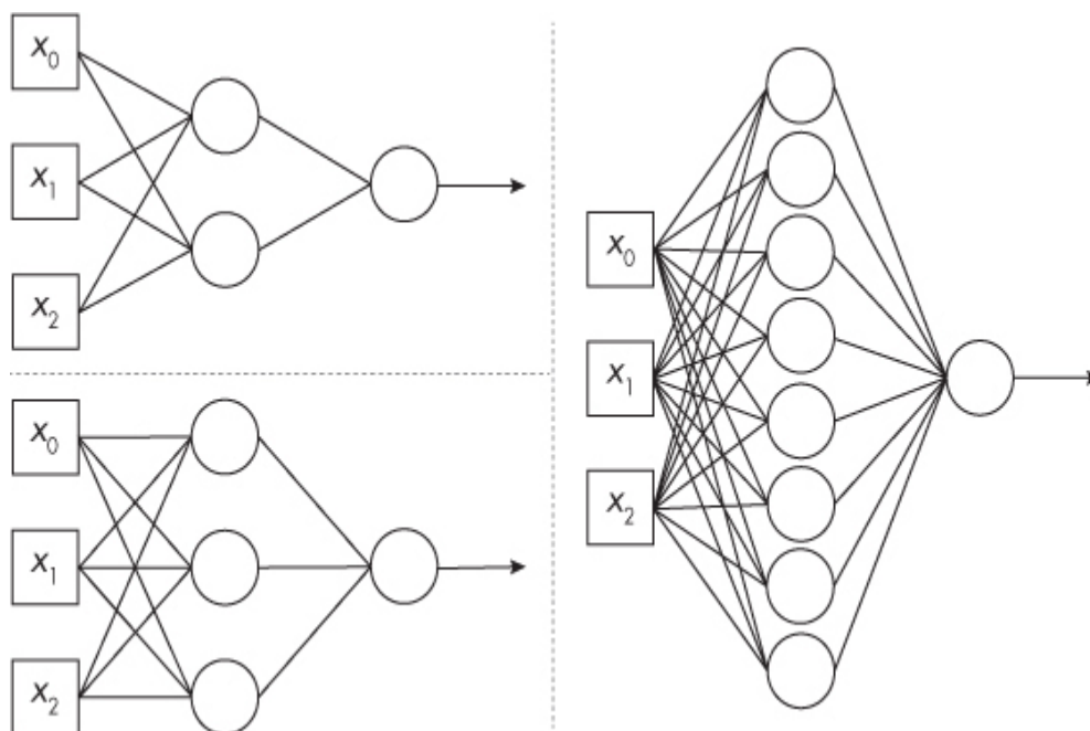
Figure 4-2: Two-, three-, and eight-node networks
