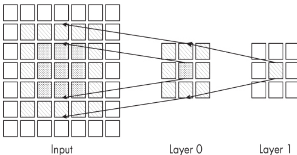
Figure 5-8: The part of the input affecting deeper layers of the model
