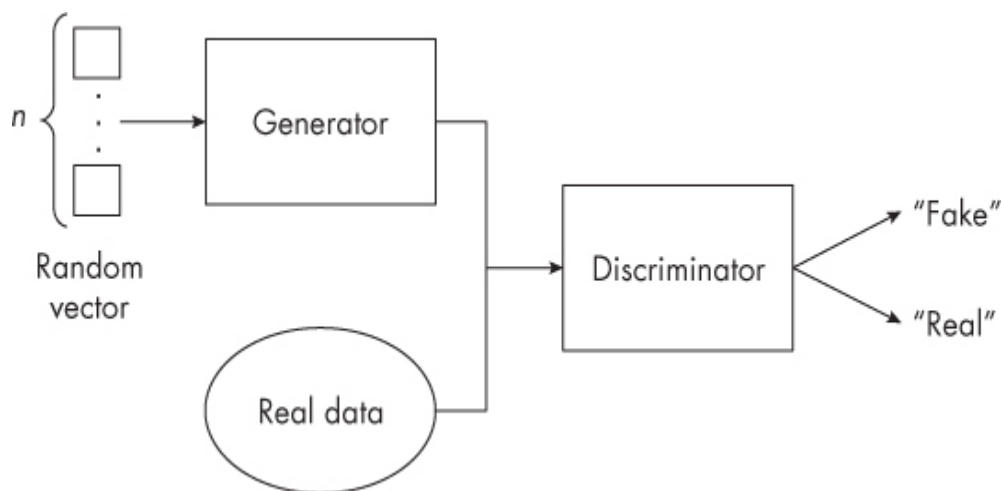
Figure 6-1: Conceptualizing the architecture of a generative adversarial network
