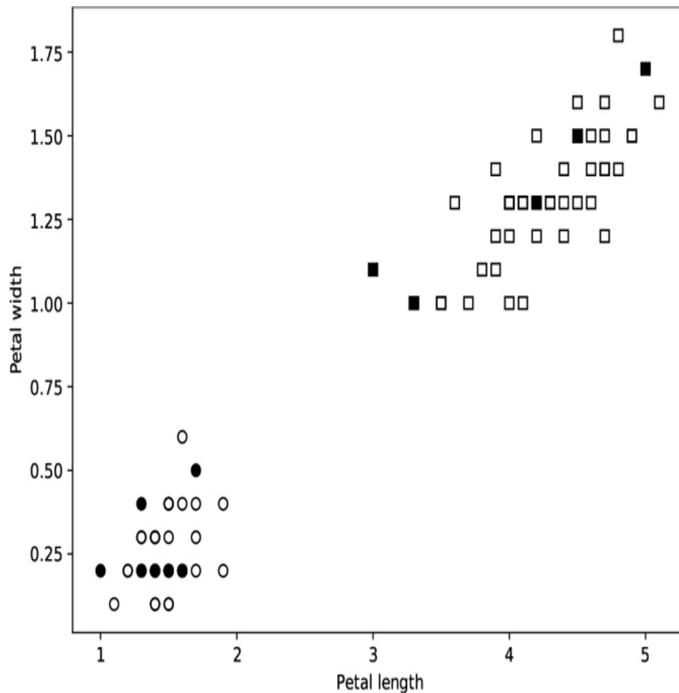
Figure 1-3: The iris training data with the held-out test data (solid)
