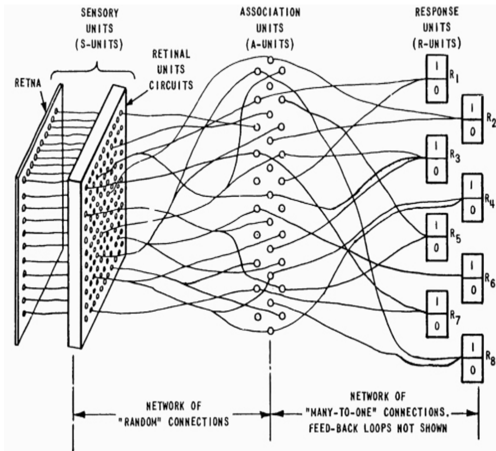
Figure 2-1: The organization of the Mark I Perceptron
