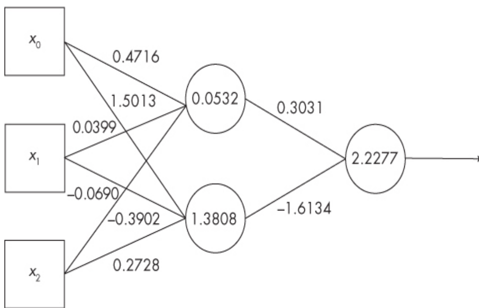
Figure 4-3: The two-neuron model trained on the wine dataset
