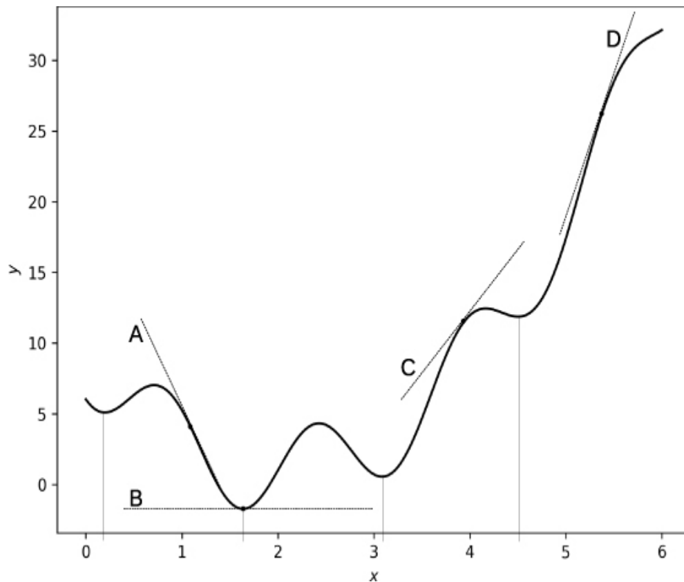
Figure 4-4: A curve with the slope at various points marked
