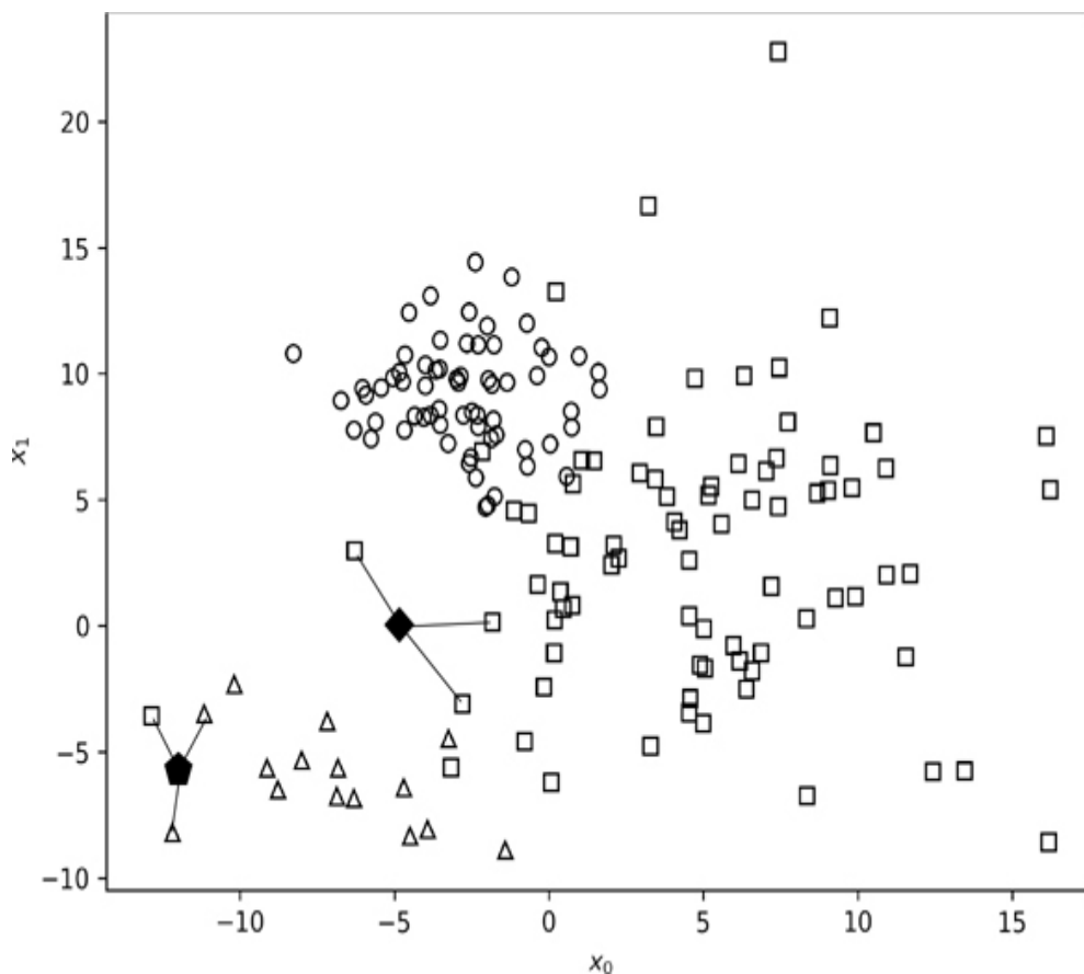
Figure 3-2: Classifying unknown samples
