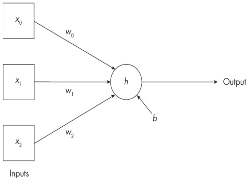
Figure 4-1: The humble (artificial) neuron
