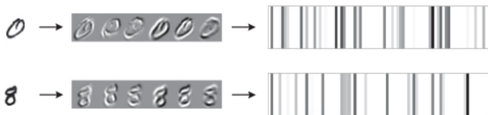
Figure 5-6: Input to first convolutional layer to dense layer
