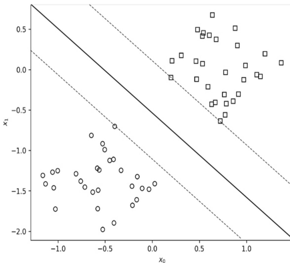
Figure 3-4: The maximal margin separating line (heavy) and maximum margins (dashed)
